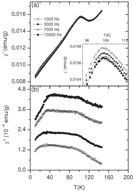
Figure 3. Temperature dependence of the real part ( \chi' ) and imaginary part ( \chi'' ) of the ac susceptibility of \text{Pr}_{0.2}\text{La}_{0.8}\text{Fe}_{11.4}\text{Al}_{1.6} , measured in a zero external dc magnetic field at typical frequencies (1000, 3000, 7000, and 10 000 Hz) during heating the sample: (a) \chi' - T and (b) \chi'' - T . The inset plot of (a) clarifies details of the real part of the ac susceptibility around 102 K. T is varied with a sweep rate of 0.25 \text{ K min}^{-1} .
