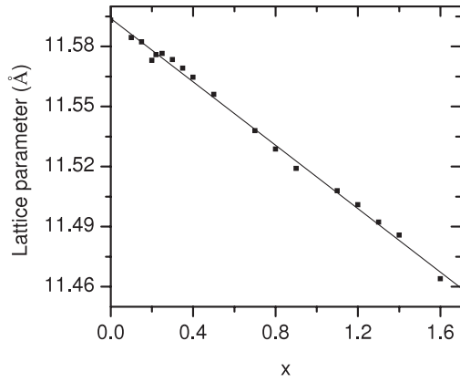
Figure 1. Si concentration dependence of the lattice parameter in \text{LaFe}_{11.4}\text{Al}_{1.6-x}\text{Si}_x ( x = 0-1.6 ) compounds. The solid line is the linear fitting result.
