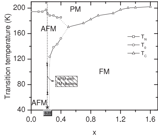
Figure 4. Magnetic phase diagram in \text{LaFe}_{11.4}\text{Al}_{1.6-x}\text{Si}_x ( x = 0-1.6 ) compounds. The solid lines and dotted lines indicate magnetic phase boundaries, and ‘ \uparrow ’ illustrates the temperature region where FM clusters appear from the AFM background for the compound with x = 0.22 . The open symbols refer to magnetic phase transition temperatures.
