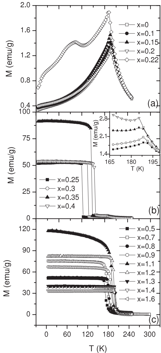
Figure 2. Temperature dependence of magnetization on heating in a field of 0.1 T of \text{LaFe}_{11.4}\text{Al}_{1.6-x}\text{Si}_x ( x = 0-1.6 ) compounds: (a) for x = 0-0.22 ; (b) for x = 0.25-0.4 ; and (c) for x = 0.5-1.6 . The inset of (b) clarifies the details in the vicinity of the AFM-PM transition for x = 0.25-0.4 .
