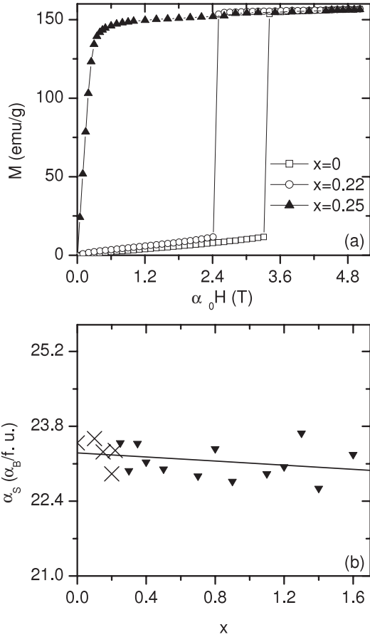
Figure 5. (a) Isothermal magnetization curves at 5 K for the selected compounds and (b) Fe concentration dependence of the saturated magnetic moments ('x' for the compounds with x \leq 0.22 and '▼' for the compounds with x \geq 0.25 ). The solid line in (b) is a guide to the eye.
