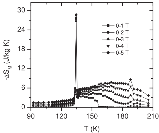
Figure 6. Temperature dependence of the magnetic entropy change -\Delta S_M of \text{LaFe}_{11.4}\text{Al}_{1.6-x}\text{Si}_x ( x = 0.3 ) compounds for typical field changes.
