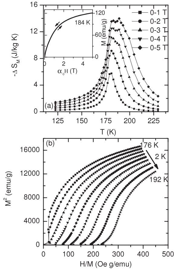
Figure 7. (a) Temperature dependence of the magnetic entropy change -\Delta S_M of \text{LaFe}_{11.4}\text{Al}_{1.6-x}\text{Si}_x ( x = 0.8 ) compounds for typical field changes and (b) Arrott-plots of this compound around T_C . Inset plot of (a): magnetization versus field curves for this compound at 184 K, arrows indicate the sequence of measurements.
